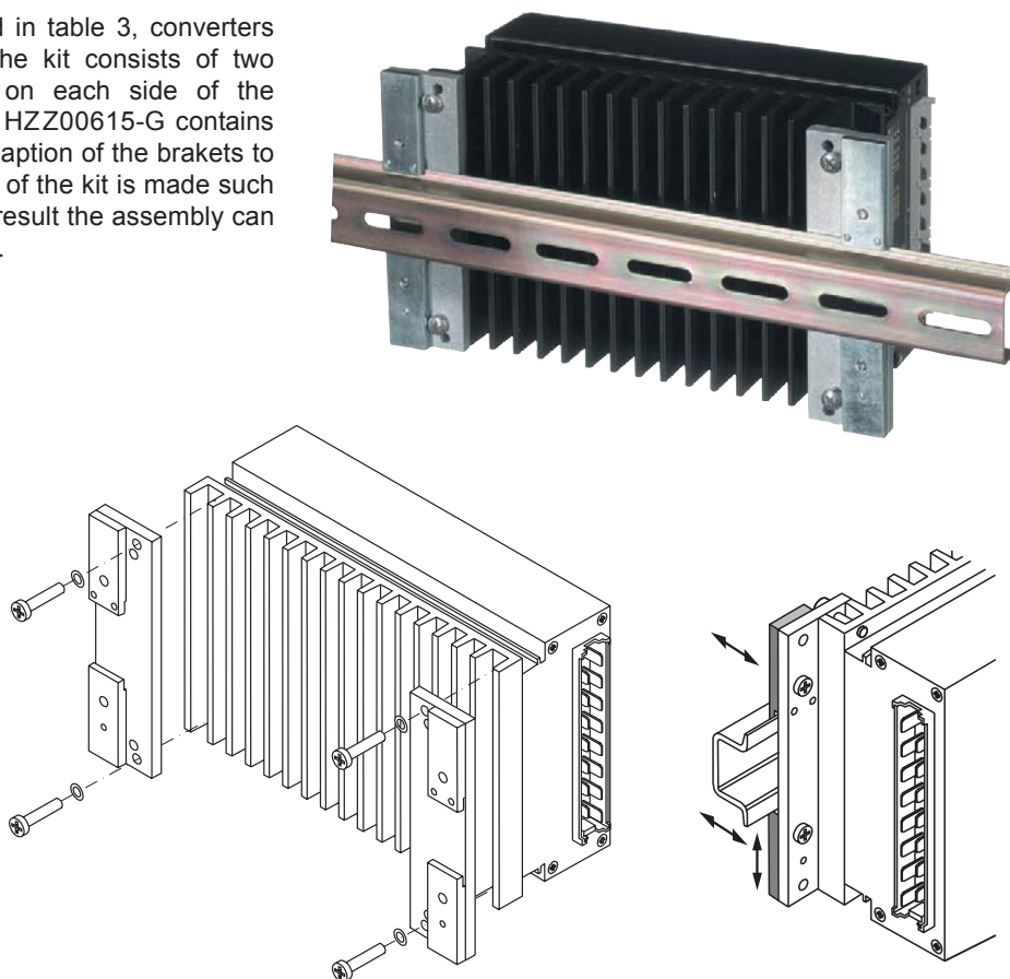
Fig. 9 Schematic view: Assembly of DMB-K/S
