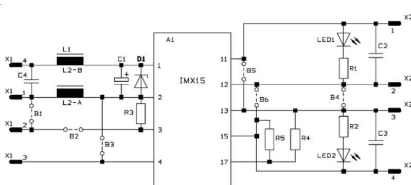
Fig. 18 C/DMB circuit diagram with IMS15, IMX15, IMY15
