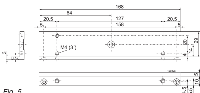
Fig. 5 Universal mounting bracket XKM159, Aluminum, untreated
