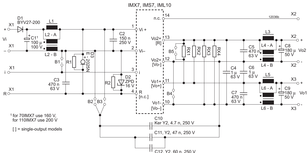
Fig. 16 C/DMB circuit diagram with IMX7, IMS7, IML10
