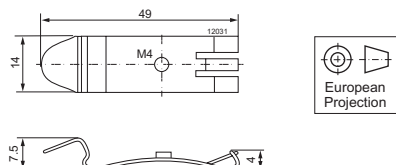
Fig. 4 DIN-rail clamp, steel, galvanized
