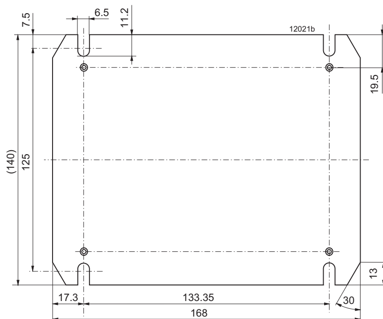
Fig. 1 HZZ01213-G (mounting plate K) Aluminum, black anodized
