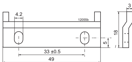
Fig. 6 Universal mounting bracket XMK038
