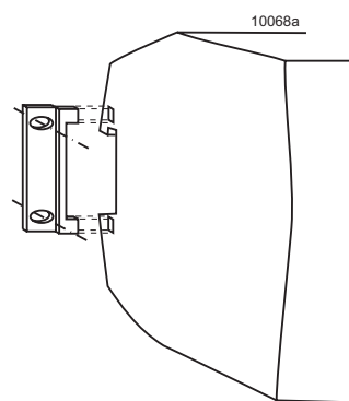
Fig. 7 W unit with chassis-mounting brackets
