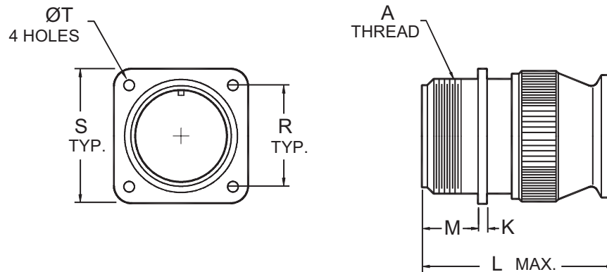
MS3100R Grommet nut, environmental, with grommet Ⓢ
