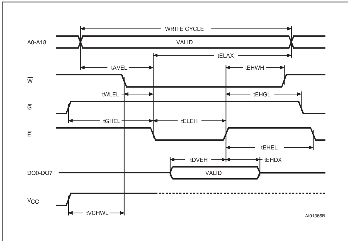
Figure 8. Write AC Waveforms, \overline{E} Controlled
