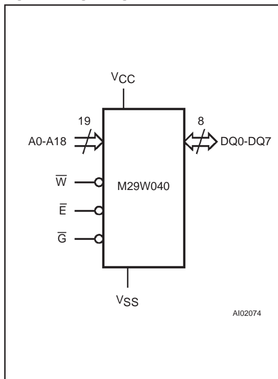
Figure 1. Logic Diagram
