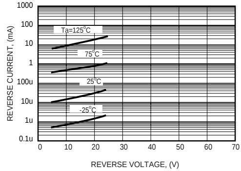
FIG. 2 - REVERSE CHARACTERISTICS
