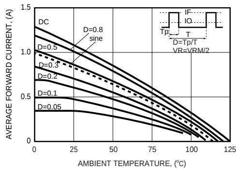
FIG. 5 - DERATING CURVE BY AMBIENT
