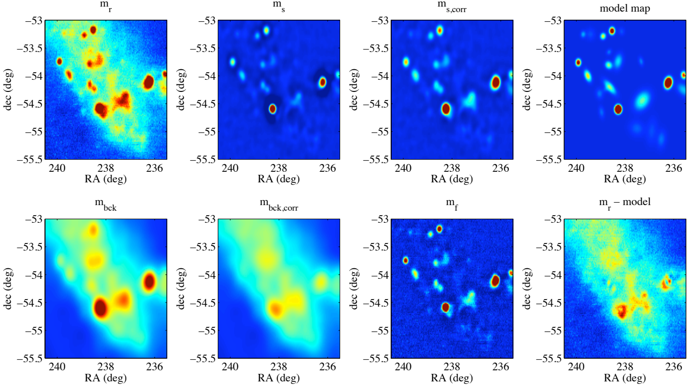
FIG. 2.— Source segmentation and fitting using a section of QUaD 100 GHz I data; colorscale is the same in all panels and runs from -0.0035 to 0.035 MJy/sr. Top Left: Raw map m_r . Bottom Left: Initial estimate of background map m_{bck} . Top row, second column: Initial background subtracted map m_s . Bottom row, second column: Background map corrected for discrete source flux ( m_{bck,corr} ). Top row, third column: Background subtracted map m_s using source-corrected background map m_{bck,corr} . Bottom row, third column: Map used for source fitting m_r - m_{bck,corr} . Top right: Model of discrete source population using fits to m_f . Bottom right: Residual between model sky and input image m_r .
