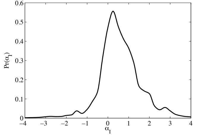
FIG. 6.— Source total intensity spectral index distribution Pr(\alpha_l) .
