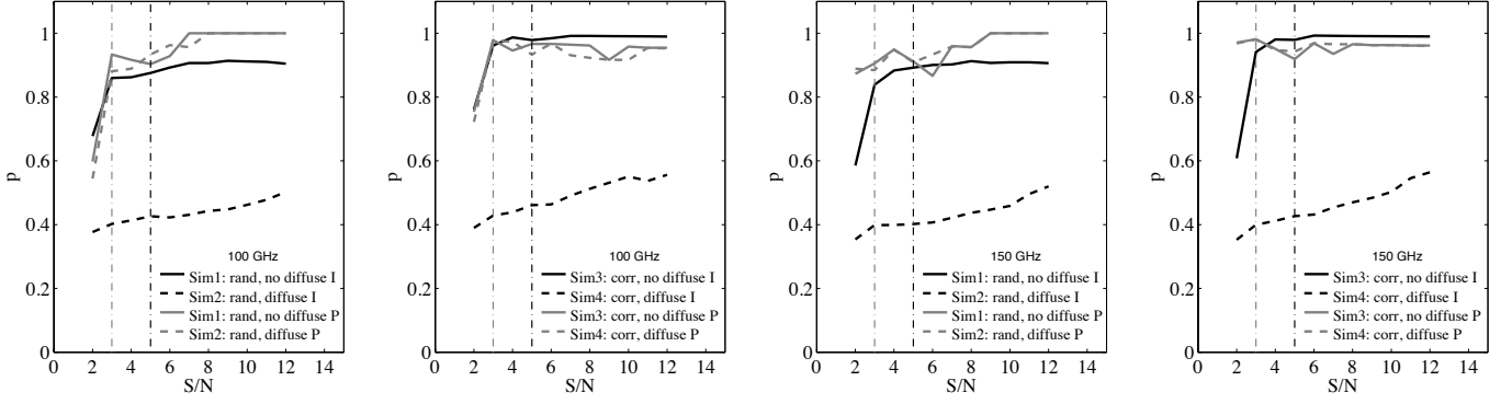
FIG. 13.— Purity as estimated from simulated point source distributions as a function of signal-to-noise (S/N). The left (right) pair of columns correspond to purity at 100 (150) GHz. Within each pair, the left plot is for randomly distributed sources with and without a diffuse background (Sim1 and Sim2), and the right plot similar but for spatially correlated sources (Sim3 and Sim4). Survey purity in total (polarized) intensity are plotted in black (gray). The vertical black dot-dashed lines correspond to the S/N ratio used to extract sources in I ; the vertical gray dot-dashed line is the same for polarization.
