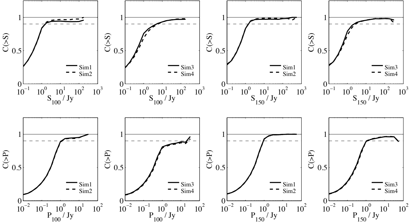
FIG. 12.— Completeness estimated from simulated point source distributions in total (top) and polarized (bottom) intensity. The left pair of columns is for 100 GHz, right pair for 150 GHz. Within each pair, the left column is for randomly distributed sources with and without a diffuse component, and likewise for spatially correlated sources in the right column. Solid black curves correspond to sources with no diffuse background present, dashed black curves are for the same source distributions with diffuse emission added. The thin dashed black line indicates 90% completeness.
