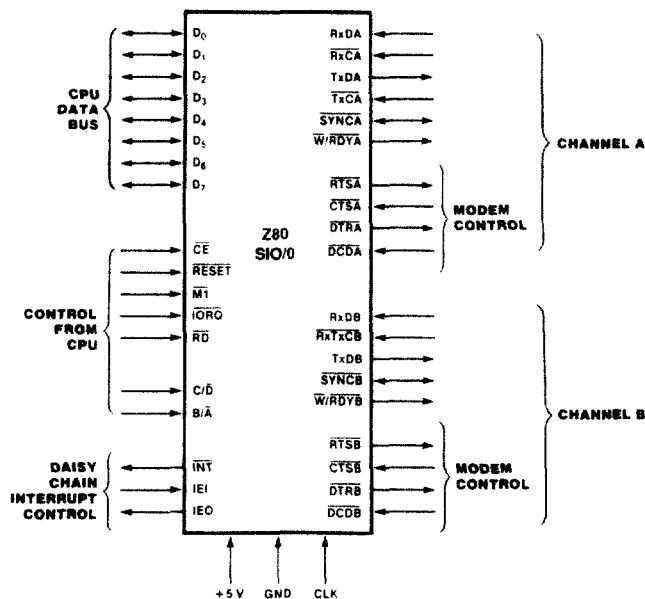
Figure 5. Pin Functions
