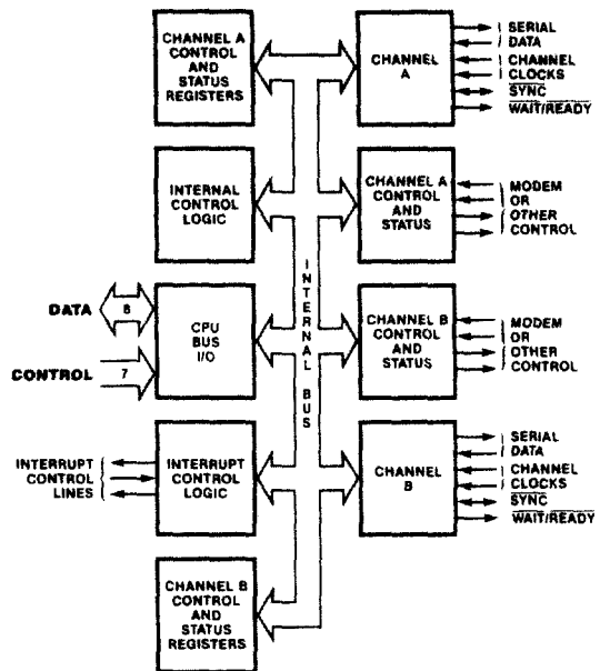
Figure 8. Block Diagram
