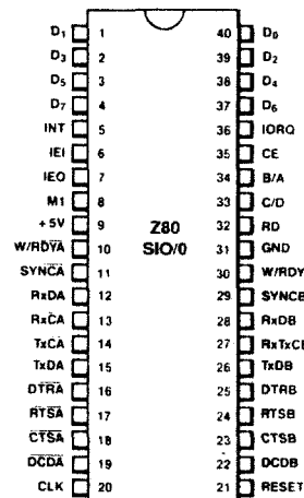
Figure 6. 40-pin Dual-In-Line Package (DIP), Pin Assignments
