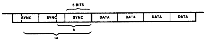
Figure 10. Data Communication
