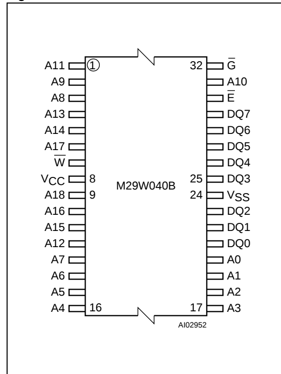
Figure 3. TSOP Connections
