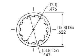
AT508 Lockwasher Steel with Zinc/Chromate
