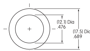
AT401P O-ring Nitrile Butadiene Rubber
