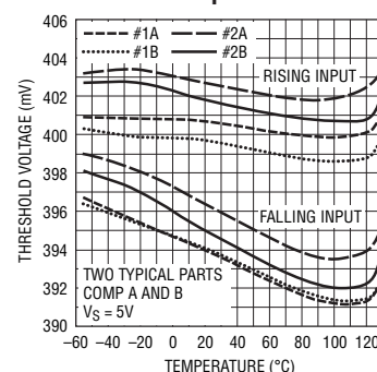
Comparator Thresholds vs Temperature
