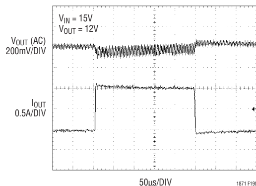
Figure 19. LTC1871 SEPIC Converter Load Step Response
