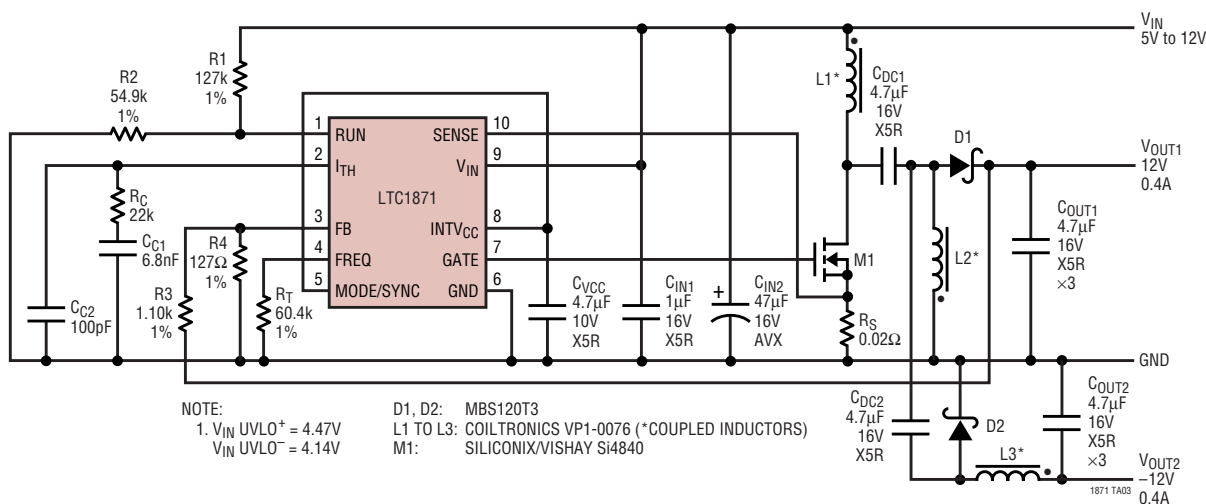
5V to 12V Input, \pm 12V/0.2A Output SEPIC Converter with Undervoltage Lockout
