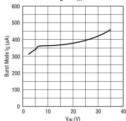
Burst Mode I_Q vs V_{IN}
