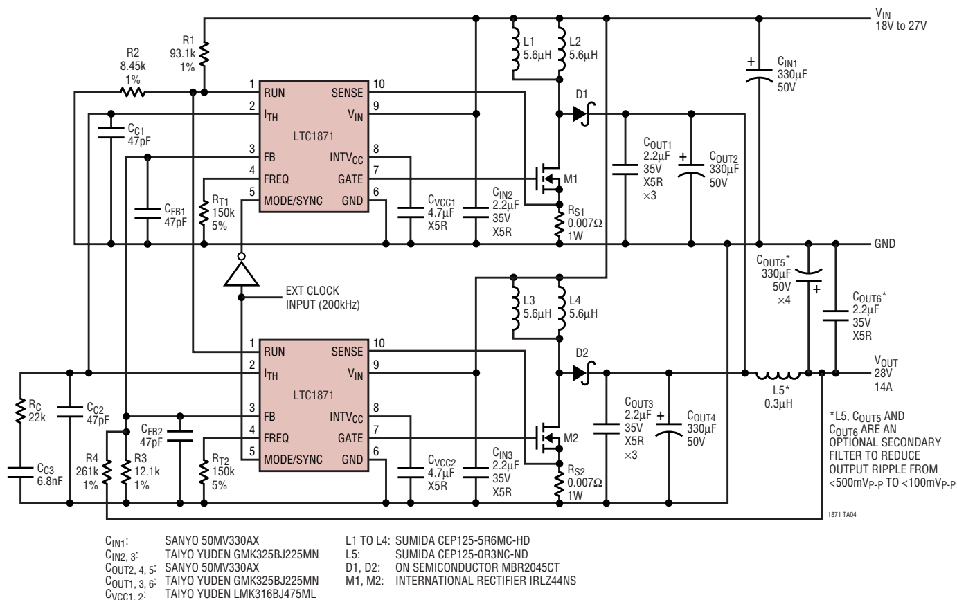
18V to 27V Input, 28V Output, 400W 2-Phase, Low Ripple, Synchronized RF Base Station Power Supply (Boost)
