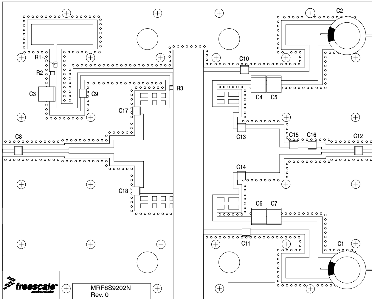
Figure 1. MRF8S9202NR3 Test Circuit Component Layout
