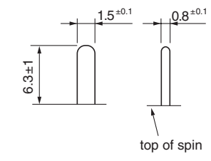
terminal dimensions
