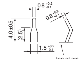
terminal dimensions
