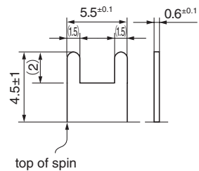
terminal dimensions
