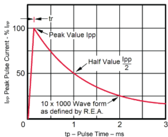
Figure 2 • Pulse Waveform
