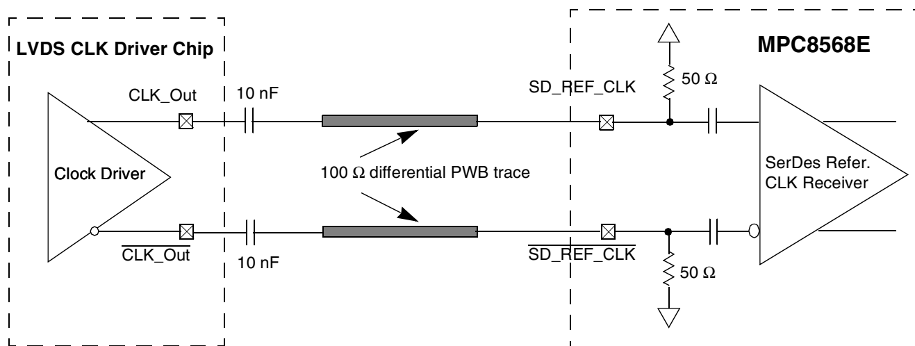
Figure 45. AC-Coupled Differential Connection with LVDS Clock Driver (Reference Only)
