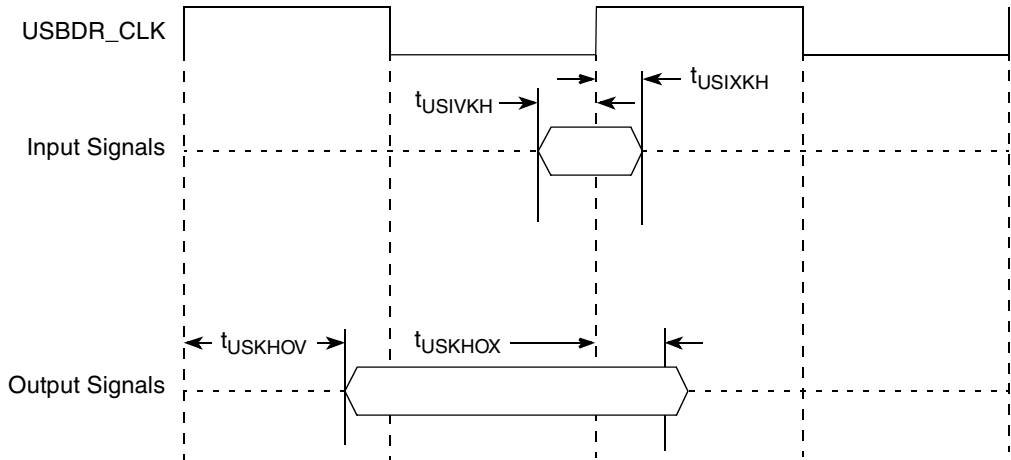
Figure 22. USB Interface Timing Diagram
