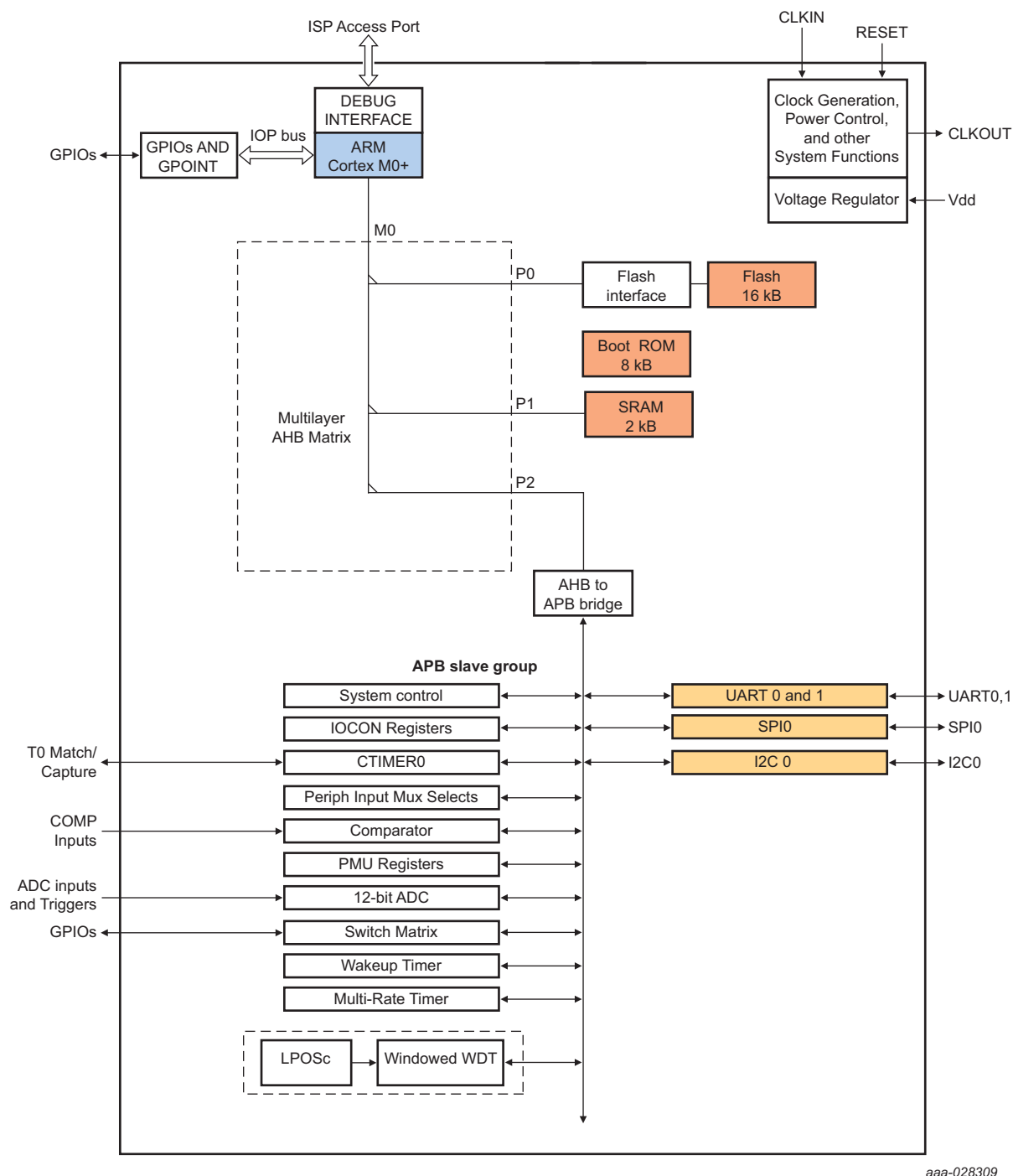
Fig 3. LPC802 block diagram
