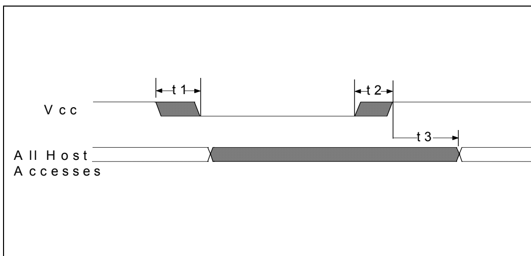
Figure 20.1 - POWER-UP TIMING
