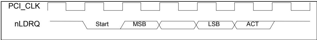
Figure 20.9 – DMA Request Assertion Through nLDRQ
