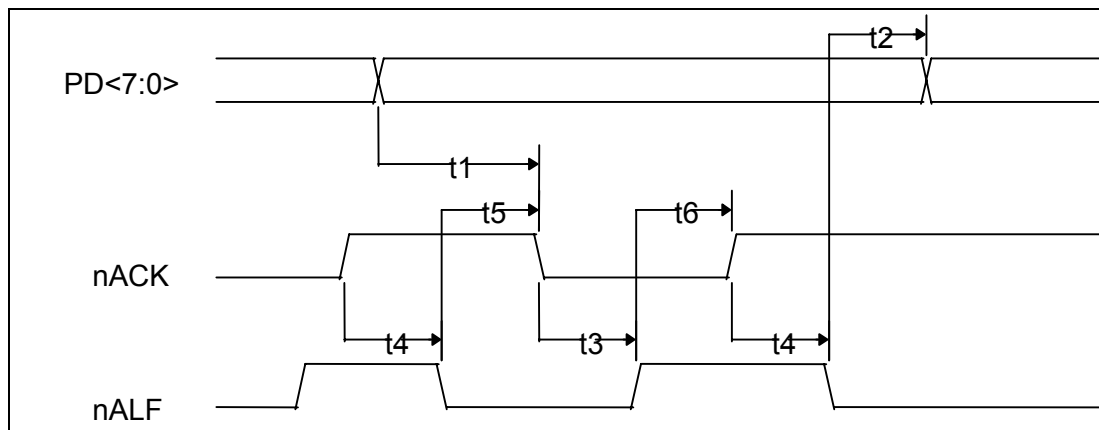
Figure 20.18 - ECP Parallel Port Reverse Timing
