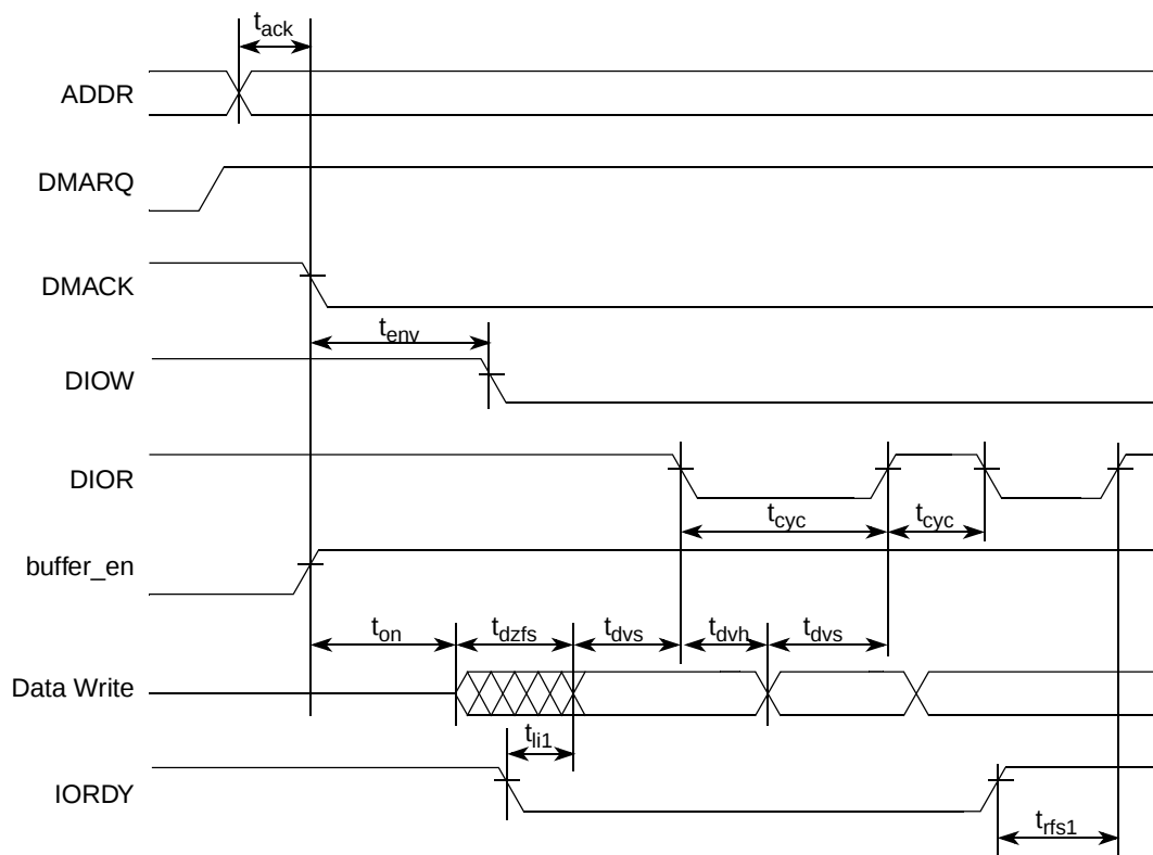
Figure 32. UDMA Out Transfer Start Timing Diagram
