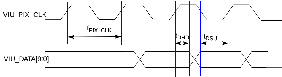
Figure 57. VIU Interface Timing Diagram
