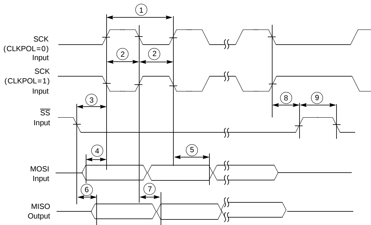
Figure 50. Timing Diagram – SPI Slave Mode, Format 0 (CPHA = 0)
