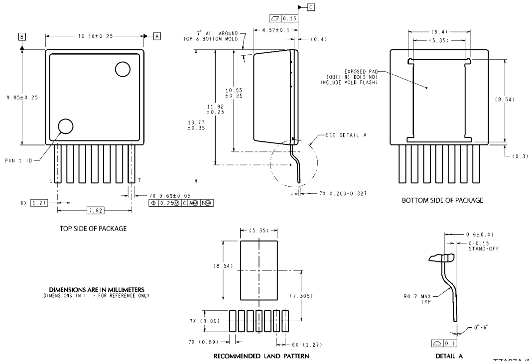
TO-PMOD-7 Pin Package NS Package Number TZA07A
