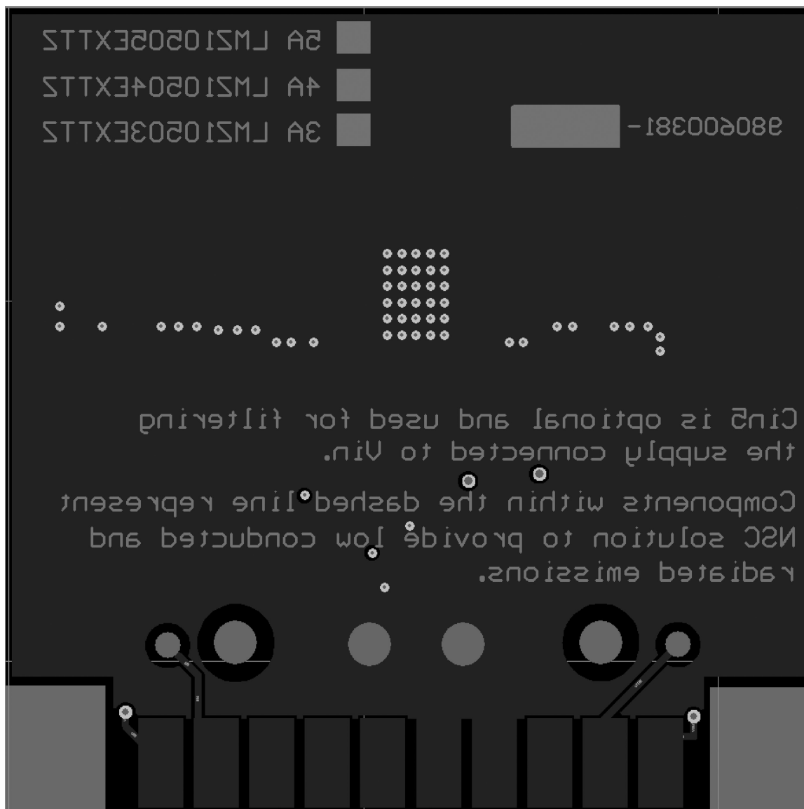
FIGURE 9. Bottom Copper
