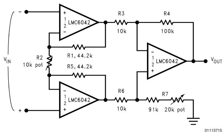
FIGURE 10. Instrumentation Amplifier
