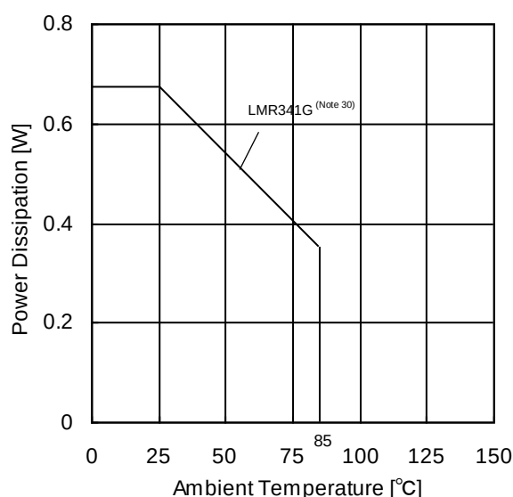
(c) LMR341G
