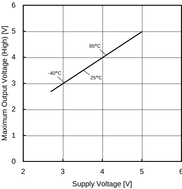
Figure 50. Maximum Output Voltage (High) vs Supply Voltage (RL=2kΩ)
