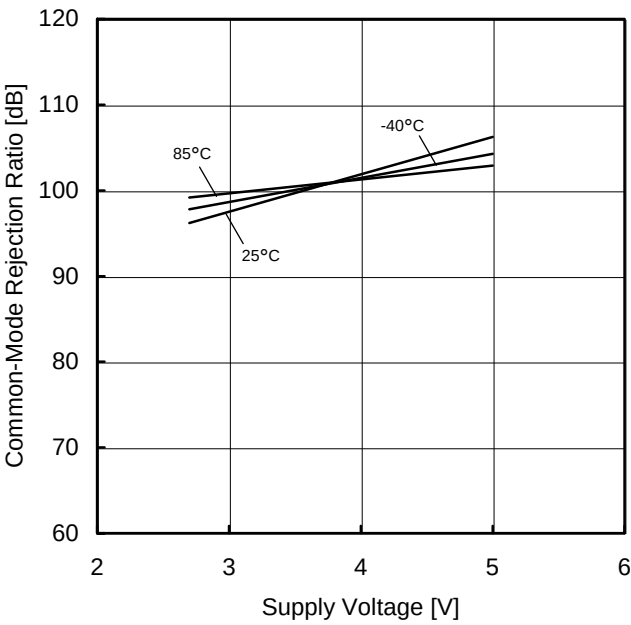
Figure 41. Common-Mode Rejection Ratio vs Supply Voltage (VDD=2.7V)
