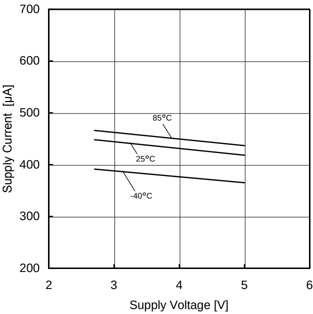
Figure 48. Supply Current vs Supply Voltage
