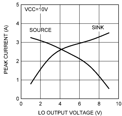
LO Peak Driver Current vs Output Voltage
