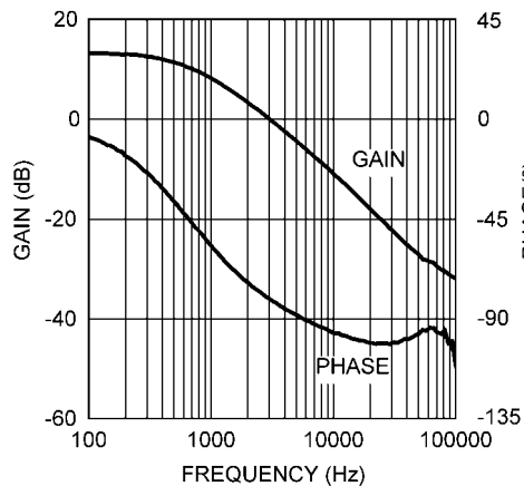
FIGURE 9. Modulator Gain and Phase
