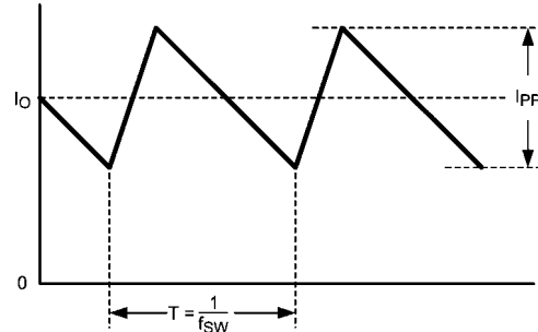
FIGURE 6. Inductor Current
