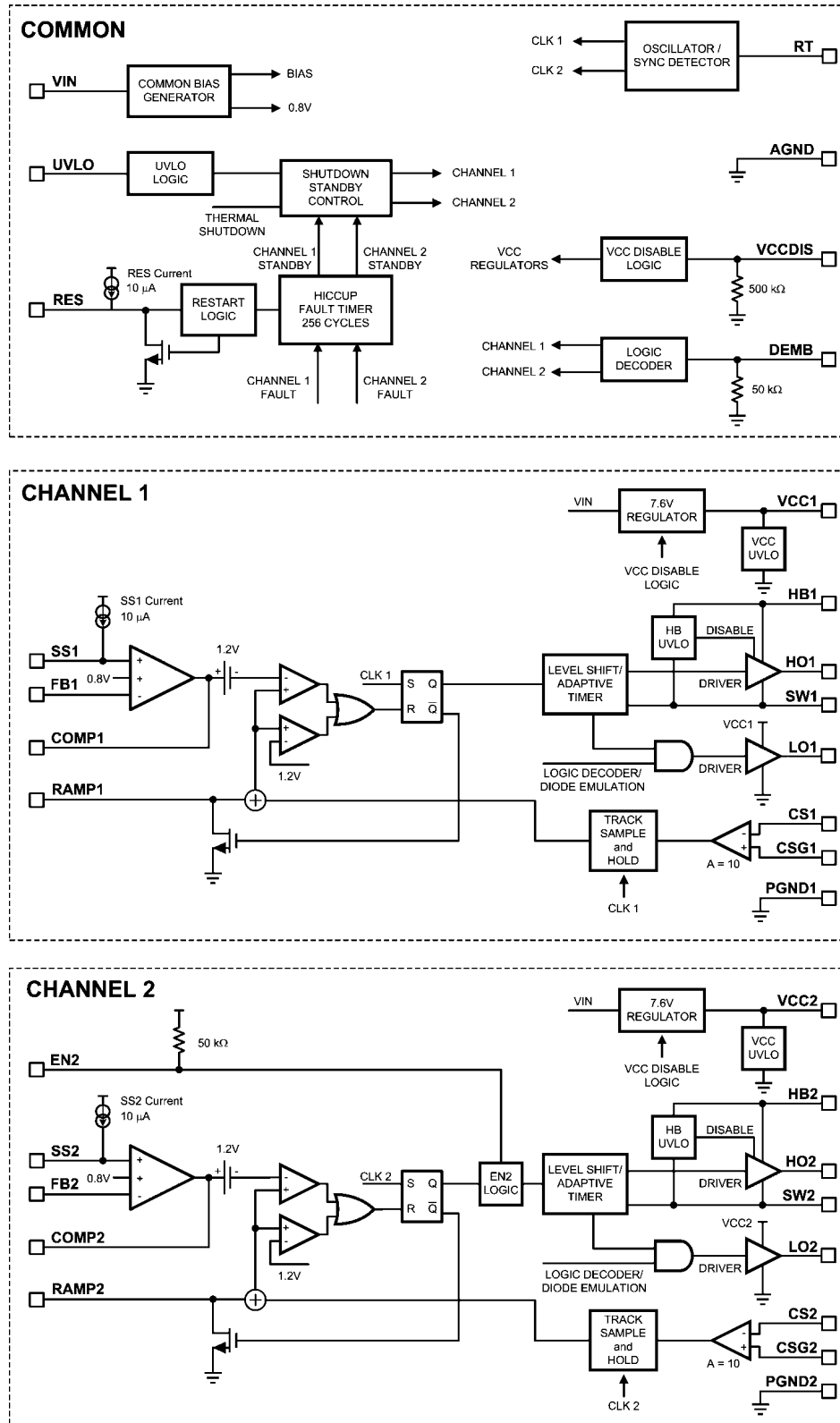
FIGURE 1. Block Diagram
