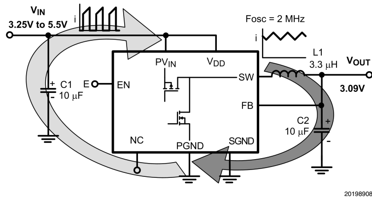
FIGURE 4. Current Loop
