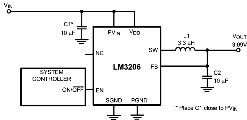
FIGURE 3. Typical Operating System Circuit
