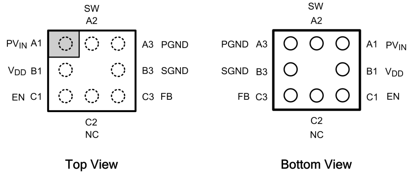
8-Bump Thin Micro SMD Package, Large Bump NS Package Number TLA08HPA
