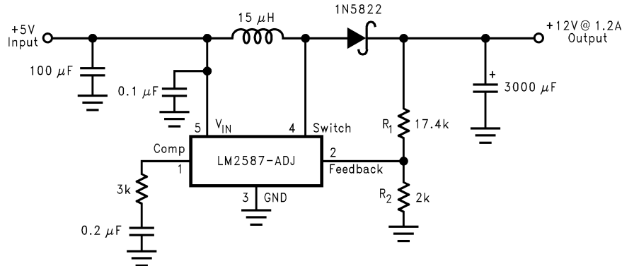
FIGURE 41. Boost Regulator
