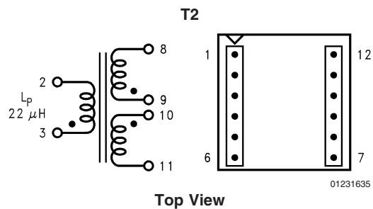
FIGURE 20. Coilcraft Q4436-B (Surface Mount)
