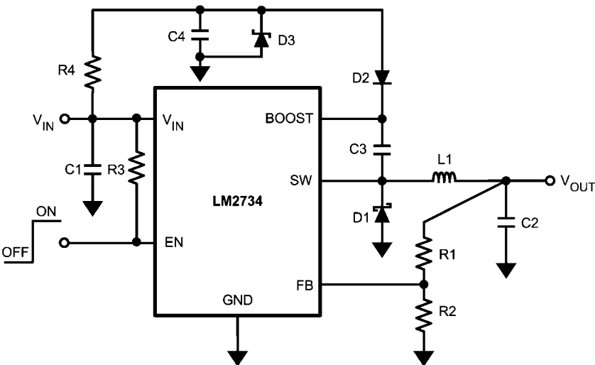
FIGURE 10. V_{\text{BOOST}} Derived from V_{\text{SHUNT}} 18V to 1.5V/1A
