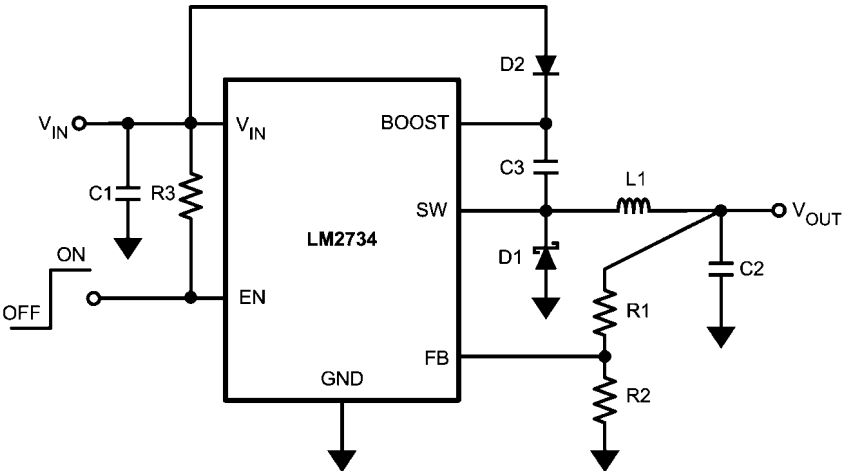
FIGURE 8. V_{BOOST} Derived from V_{IN} Operating Conditions: 5V to 1.5V/1A
