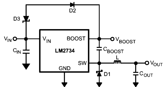
FIGURE 4. Zener Reduces Boost Voltage from V_{IN}
