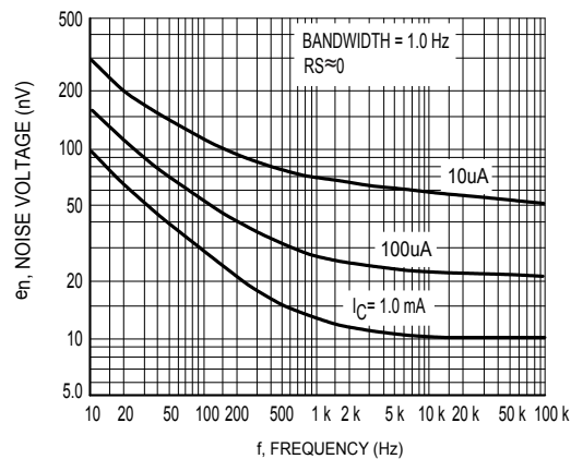
Figure 1 Noise Voltage
