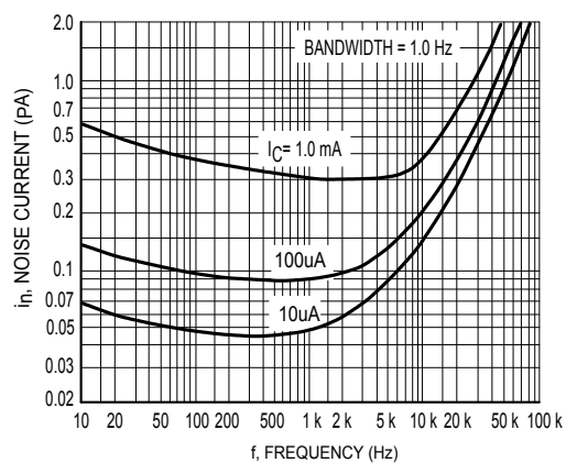
Figure 2 Noise Current
