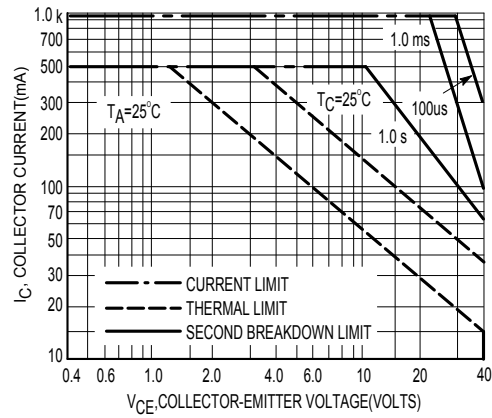
Figure 12 Active Region Safe Operating Area
