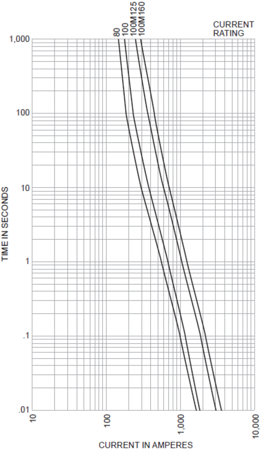
Time-Current Characteristic Curve (Full Size Curves Available)
