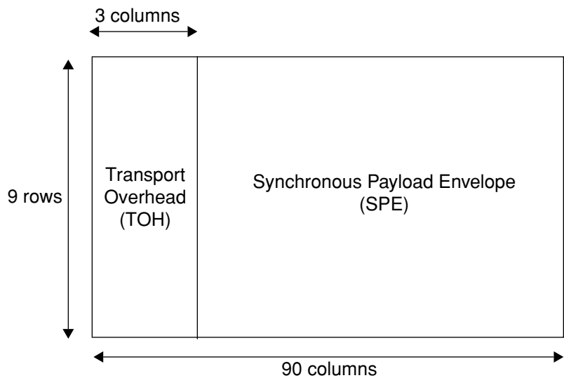
Figure 4. STS-1 Frame Format
