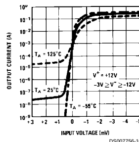
Transconductance
