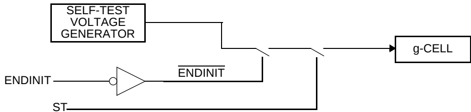
Figure 10. Self-test Interface
