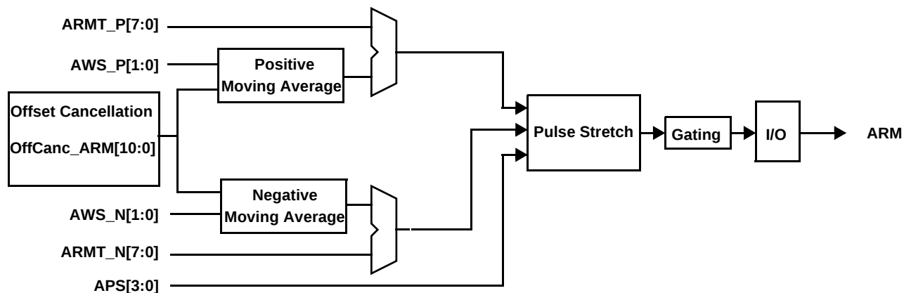
Figure 25. Arming Function Block Diagram - Moving Average Mode
