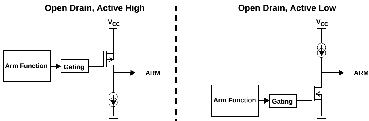
Figure 30. Arming Function - Pin Output Structure
