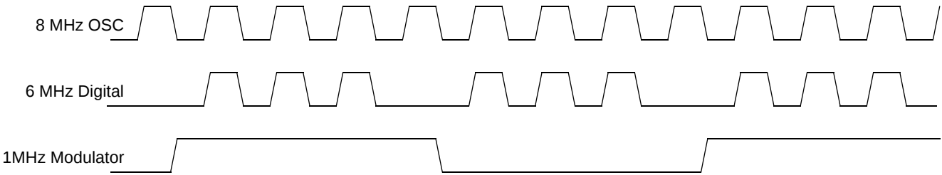
Figure 13. Clock Generation
