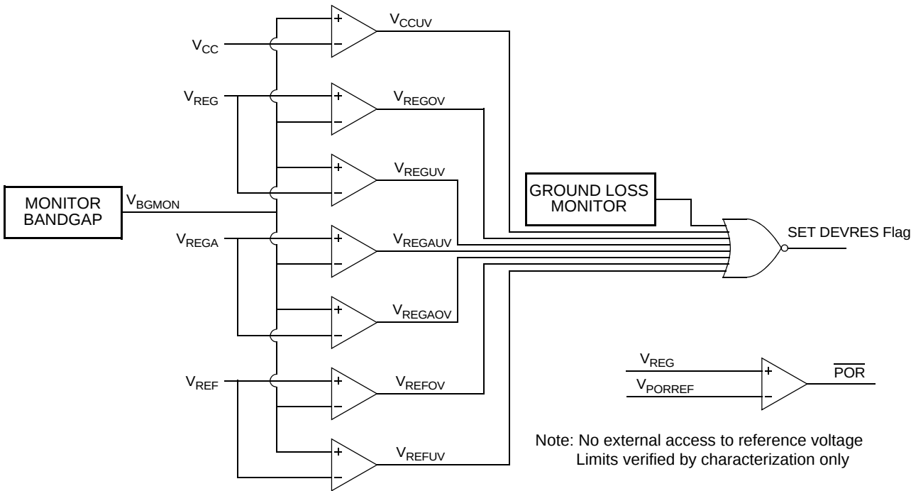
Figure 9. Voltage Monitoring
