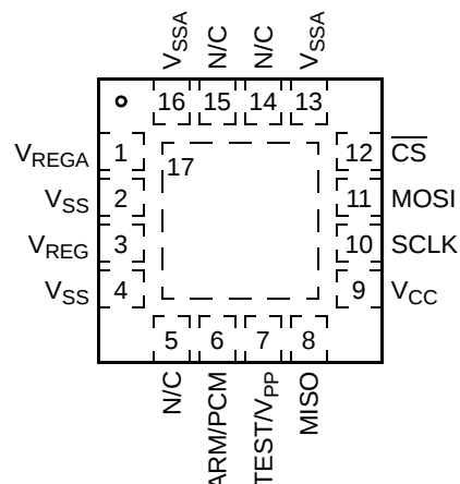
Pin Connections
