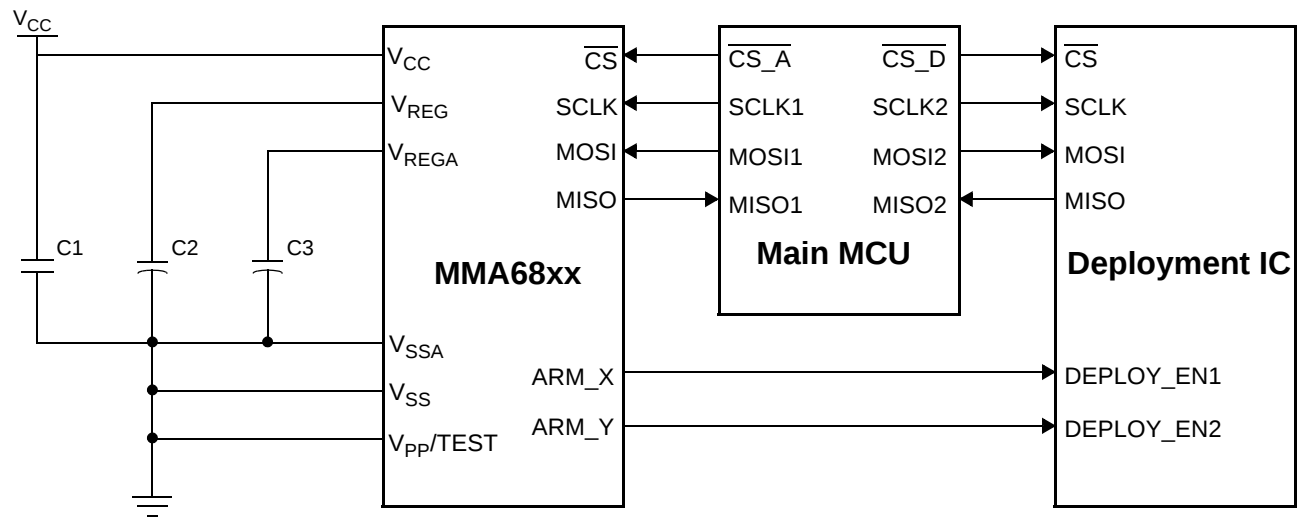
Figure 1. Application Diagram
