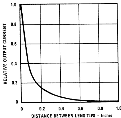
Coupling Characteristics of OP145 and OP555
