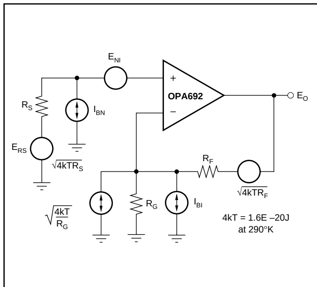
FIGURE 8. Noise Model.
