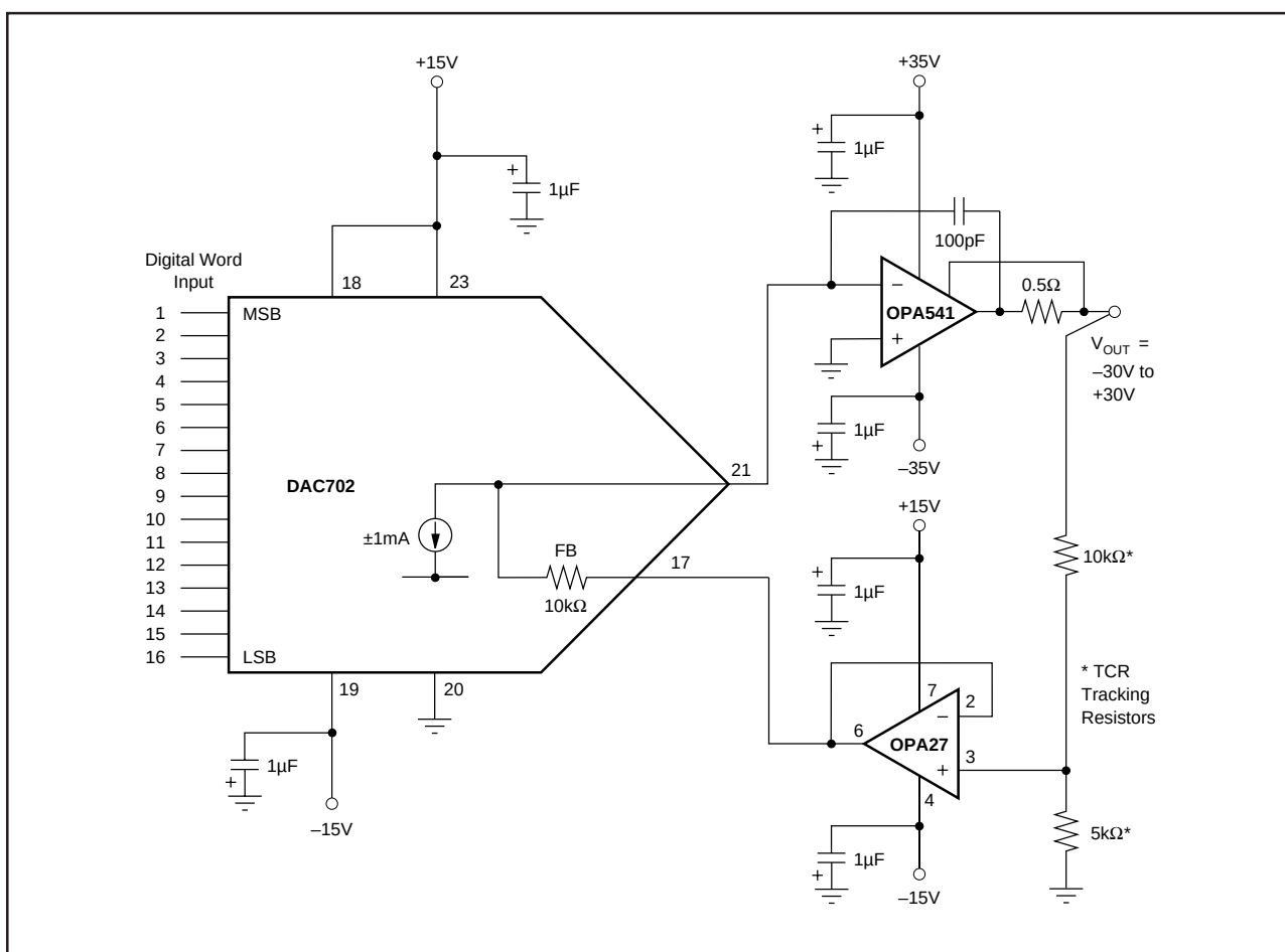
FIGURE 7. 16-Bit Programmable Voltage Source.
