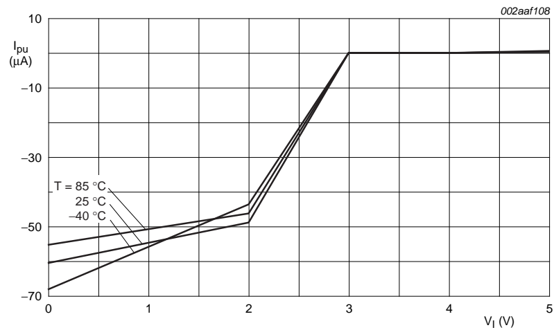
Fig 13. Typical pull-up current I_{pu} versus input voltage V_i
