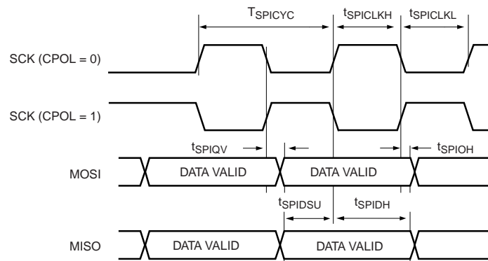
Fig 23. SPI master timing (CPHA = 0)
