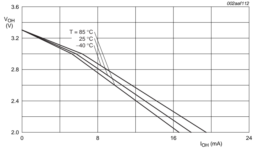
Fig 11. Typical HIGH-level output voltage V_{OH} versus HIGH-level output source current I_{OH}
