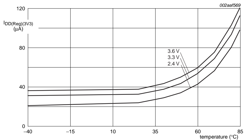
Fig 8. Power-down mode: Typical regulator supply current I_{DD(REG)(3V3)} versus temperature
