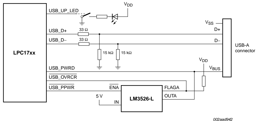
Fig 31. USB host port configuration
