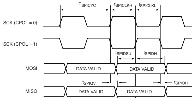
Fig 24. SPI slave timing (CPHA = 1)
