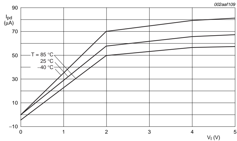
Fig 14. Typical pull-down current I_{pd} versus input voltage V_i
