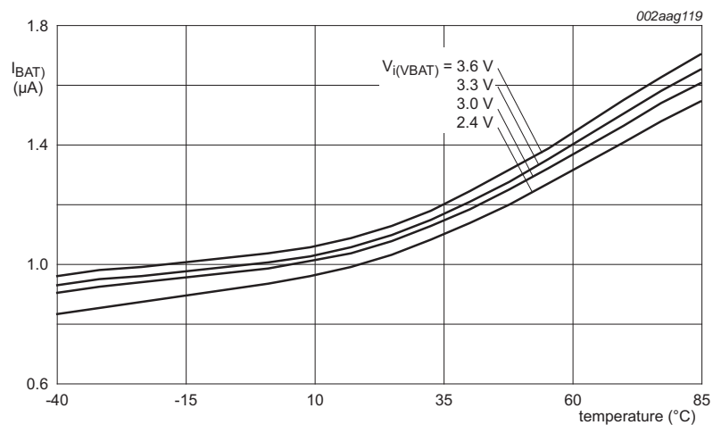
Fig 9. Deep power-down mode: Typical battery supply current I_{BAT} versus temperature
