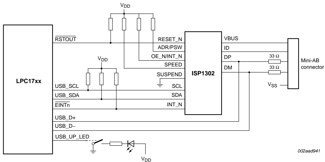
Fig 30. USB OTG port configuration
