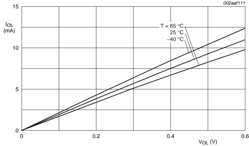
Fig 12. Typical LOW-level output current I_{OL} versus LOW-level output voltage V_{OL}
