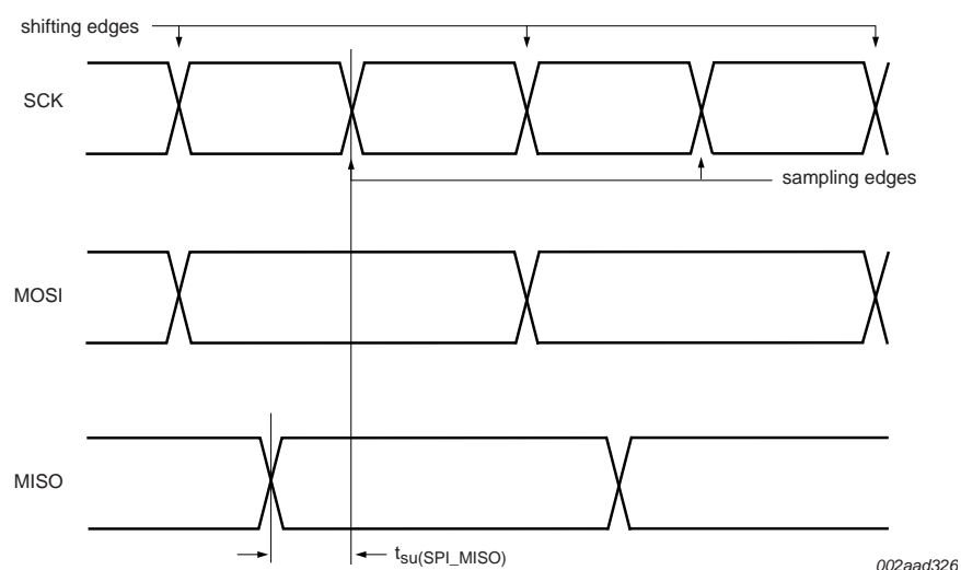
Fig 20. MISO line set-up time in SSP Master mode
