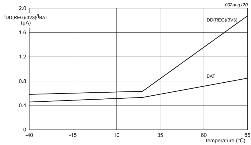
Fig 10. Deep power-down mode: Typical regulator supply current I_{DD(REG)(3V3)} and battery supply current I_{BAT} versus temperature
