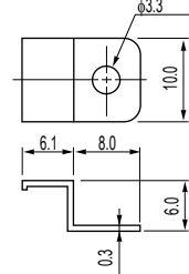
OHD1 Mounting Bracket
