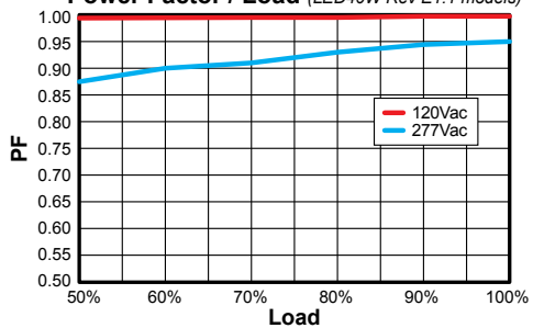
Power Factor / Load (LED40W Rev E1.1 models)
