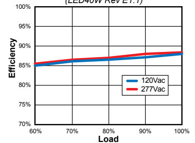
Typical Efficiency / Load (LED40W Rev E1.1)
