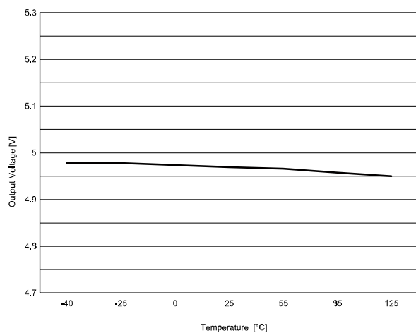
Figure 7. Output voltage vs. temperature ( V_{IN} = 6\text{ V} , V_{OUT} = 5\text{ V} , 1200 mA)
