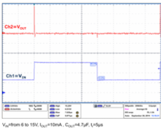
Figure 24. Line transient ( V_{OUT} = 5\text{ V} )
