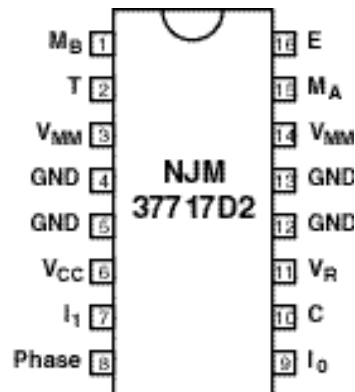
Figure 2. Pin configurations
