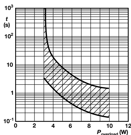
NFR25 This graph is based on measured data which may deviate according to the application. Fusing Characteristics: 1 \Omega \leq R \leq 15 \Omega
