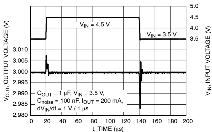
Figure 33. Line Transient Response, V_{OUT} = 3.0 V , C_{OUT} = 1 \mu F , I_{OUT} = 200 mA
