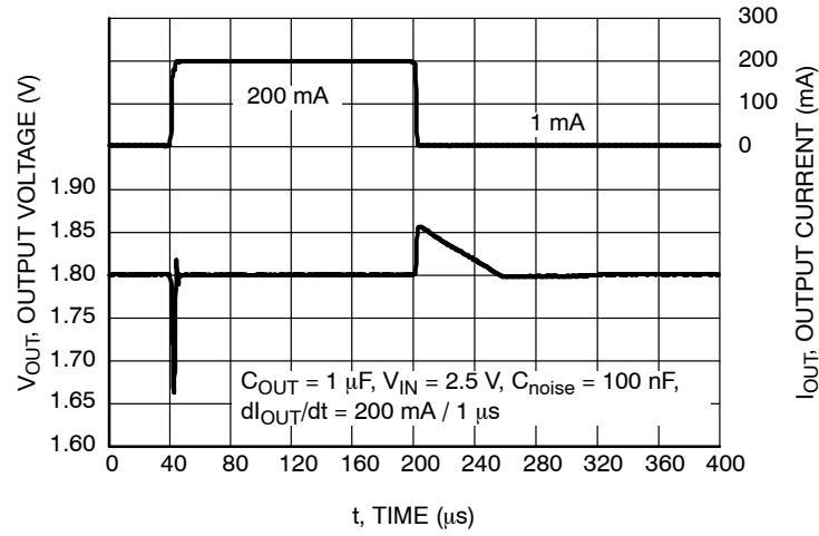
Figure 27. Load Transient Response, V_{OUT} = 1.8\text{ V} , C_{OUT} = 1\text{ }\mu\text{F} , C_{noise} = 100\text{ nF}
