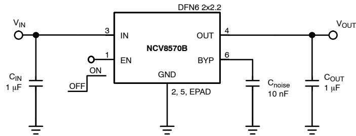
Figure 1. NCV8570B Typical Application Schematic
