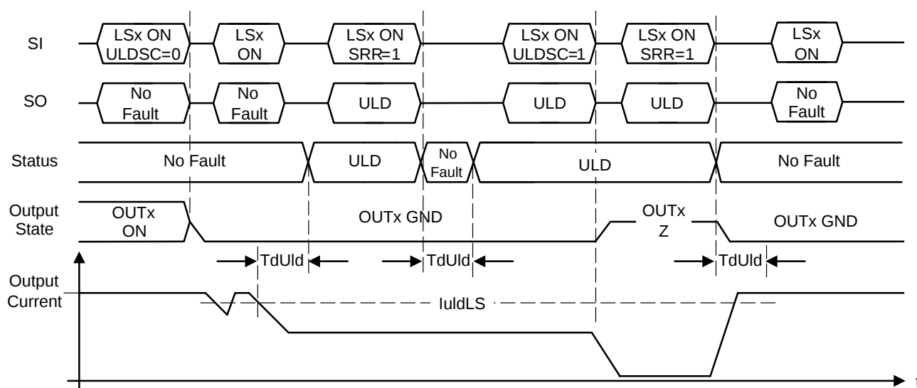
Figure 22. Underload Timing
