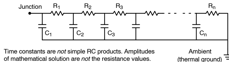
Figure 29. Grounded Capacitor Thermal Network ("Cauer" Ladder)
