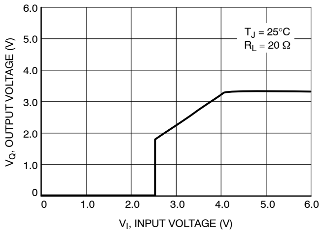
Figure 12. Low Voltage Behavior, 3.3 V Version
