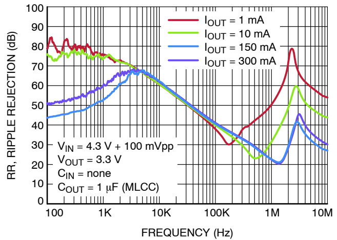
Figure 27. Power Supply Rejection Ratio, V_{OUT} = 3.3 V
