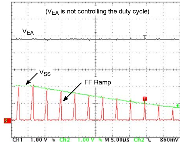
Figure 34. Soft-Stop Before Soft-Start is Complete and V_{\text{EA}} is Open.
