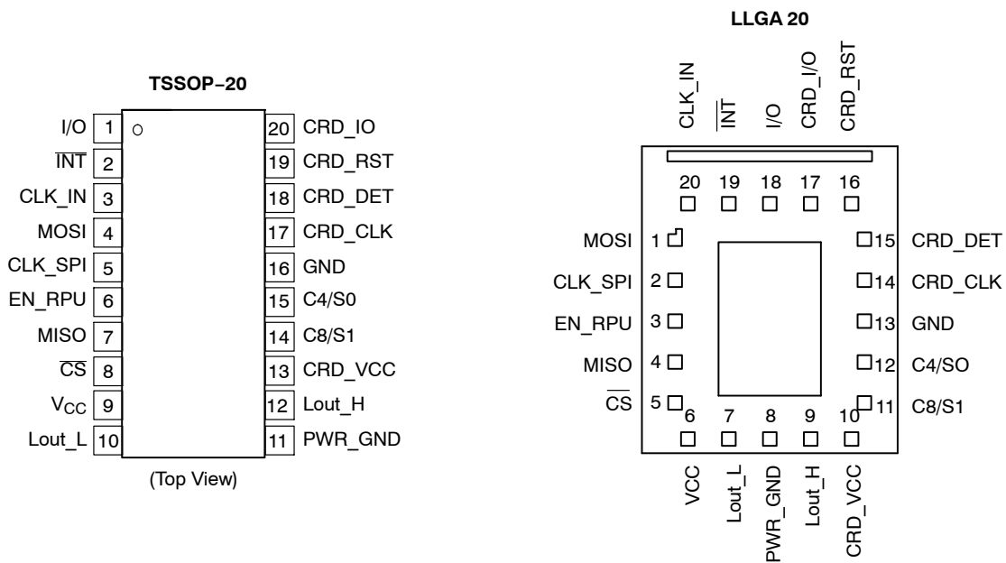
Figure 1. Pin Connections*
