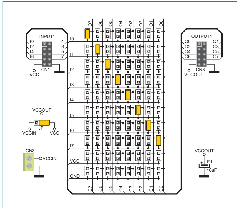
Figure 4: Smart ADAPT board connection schematic
