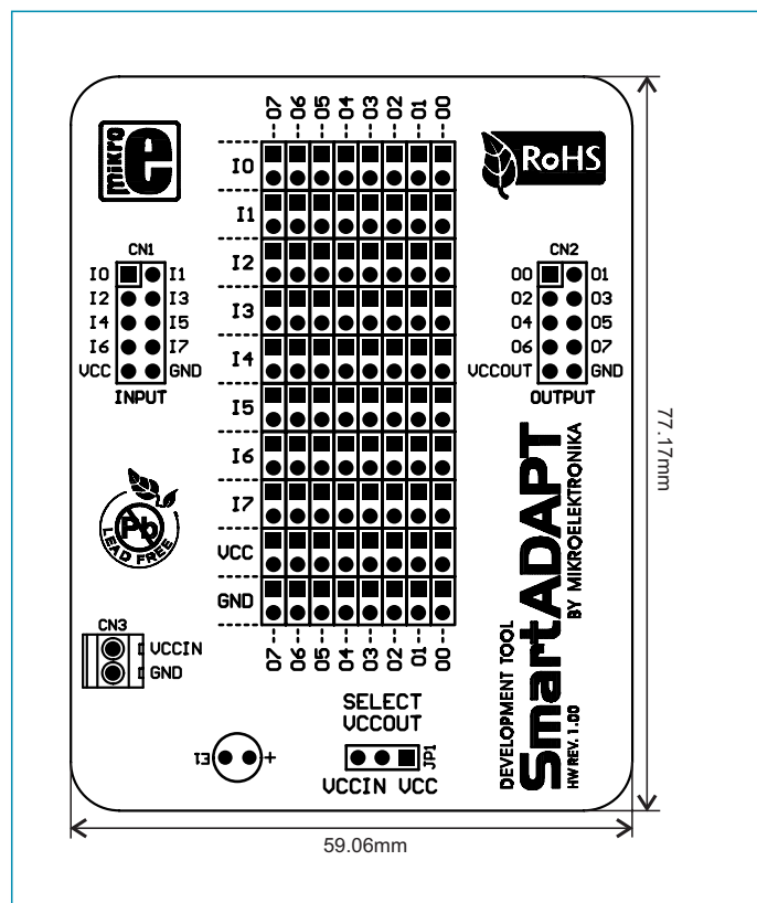
Figure 5: Dimensions of the Smart ADAPT board
