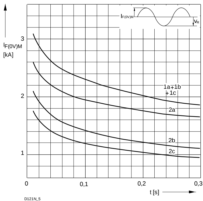
Bild / Fig. 3 Grenzstrom / Maximum overload forward current I_{F(0V)M} = f(t) 1 - I_{FAV(vor)} = 0\text{ A} ; t_{vj} = t_c = 25\text{ °C} 2 - I_{FAV(vor)} = 120\text{ A} ; t_c = 113\text{ °C} ; t_{vj} = 180\text{ °C} a - V_R \leq 50\text{ V} b - V_R = 0,5\text{ V RRM} c - V_R = 0,8\text{ V RRM}
