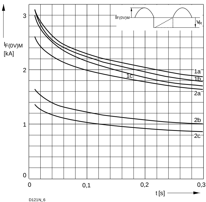
Bild / Fig. 4 Grenzstrom / Maximum overload forward current I_{F(0V)M} = f(t) 1 - I_{FAV(vor)} = 0\text{ A} ; t_{vj} = t_c = 25\text{ °C} 2 - I_{FAV(vor)} = 120\text{ A} ; t_c = 113\text{ °C} ; t_{vj} = 180\text{ °C} a - V_R \leq 50\text{ V} b - V_R = 0,5\text{ V RRM} c - V_R = 0,8\text{ V RRM}
