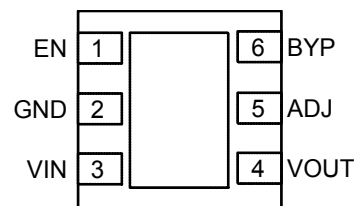
MIC5319BML/YML (Adjustable) 6-Pin 2mm x 2mm MLF™ (ML) (Top View)
