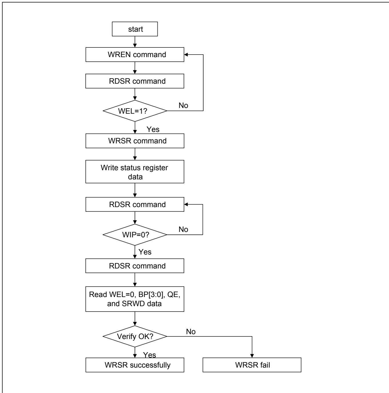
Figure 14. WRSR flow
