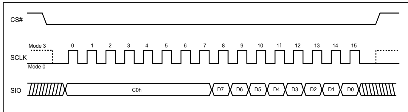
Figure 22. Burst Read
